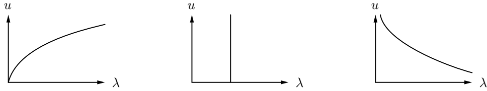
FIGURE 1. Bifurcation Diagrams: (a) sublinear; (b) “linear”; (c) superlinear
